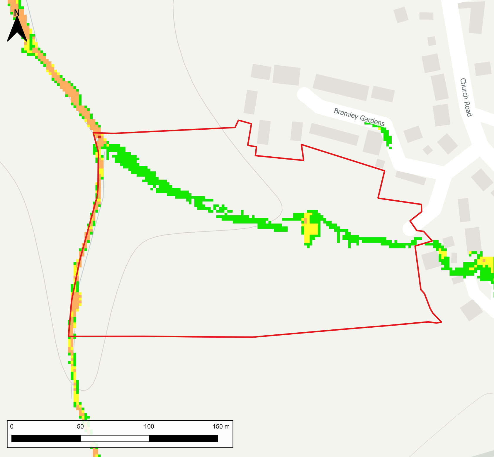
Surface Water 3.3% AEP plus 65% Climate Change
