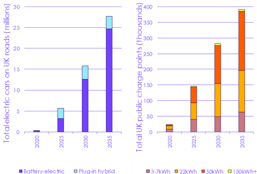
Figure A3.1.b Total electric cars on the road and supporting charging infrastructure in the Balanced Net Zero Pathway
